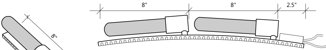
ELEVATION DIAGRAM NOT TO SCALE
